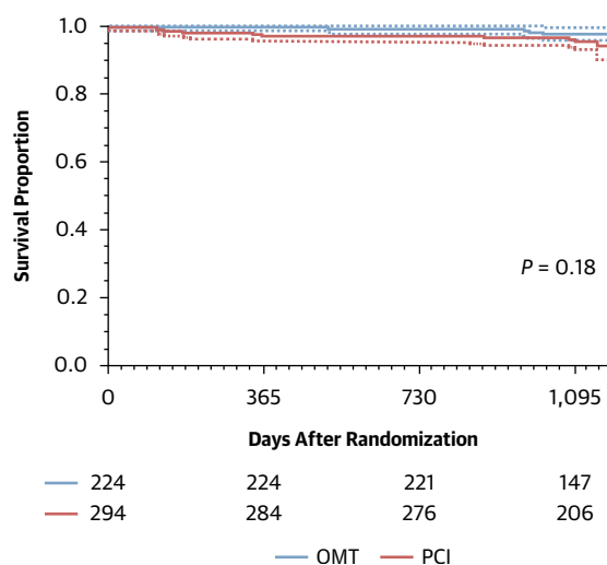
FIGURE 5 Survival Free of Death and Nonfatal MI With OMT or PCI
